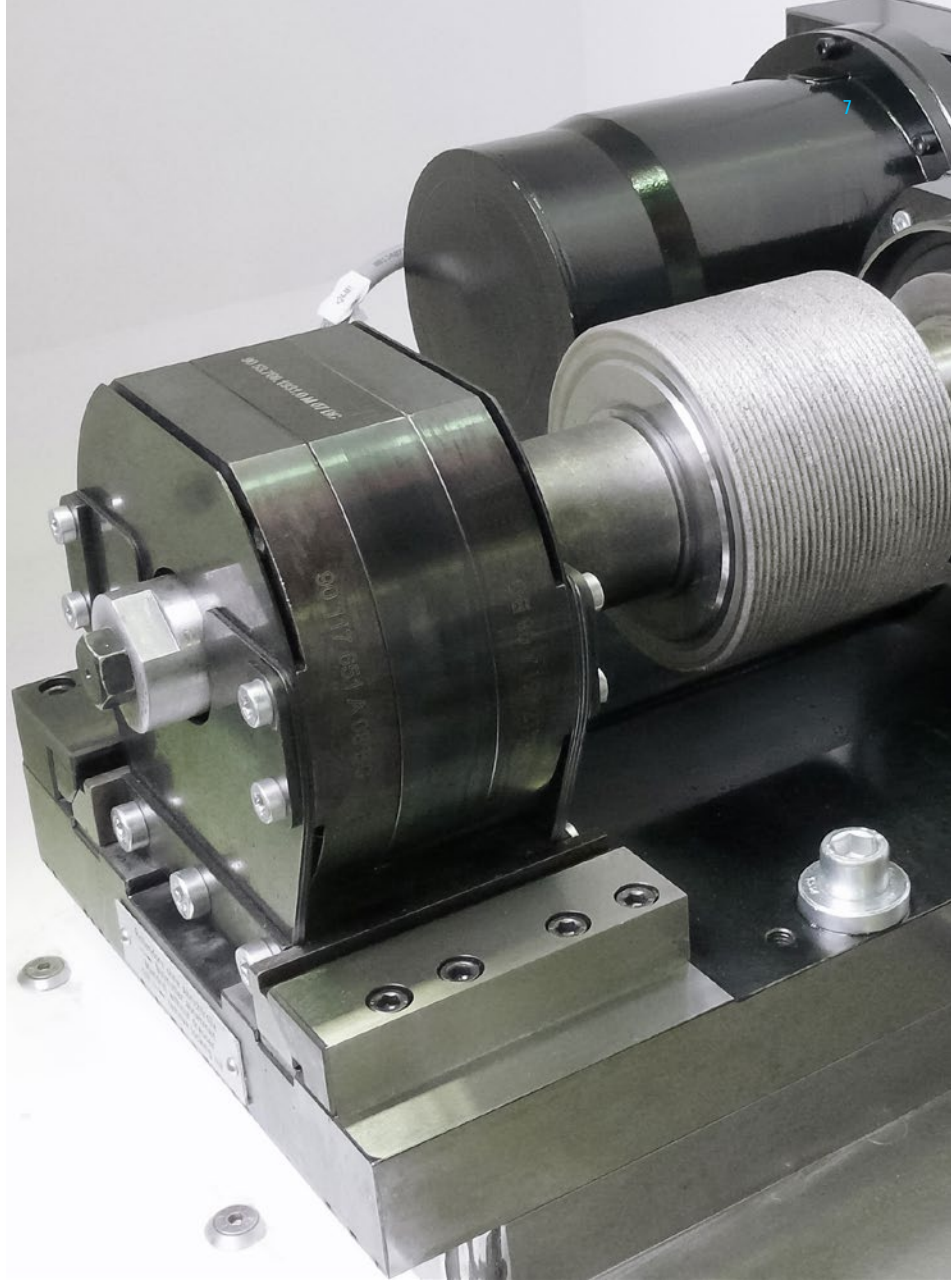
▲ Table mounted dresser type PA-TL 200S for diamond rolls up to a width of 200 mm or for contour dressing with universal diamond dressing discs and a rough dressing disc.
